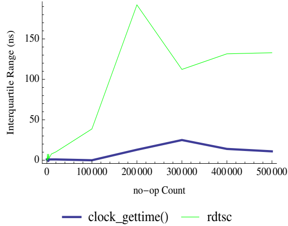
Figure 5.4: Interquartile range difference ( IQRD = 75^{th} - 25^{th} ) in nanoseconds for the times measured for each set of “no-op” instructions (number instructions listed on x-axis). Each instruction length was executed 10^6 \times for each method. The IQR gives a visual representation to the stability of measurements for these two timing methods.
