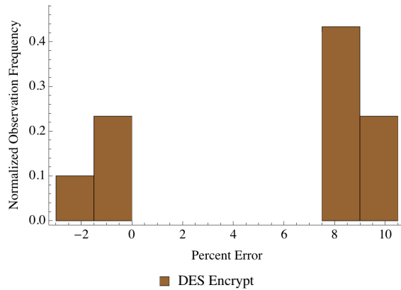
Figure 4.13: Percent error for gain/loss flow model for the DES encrypt application, calculated as \frac{(\text{observed flow} - \text{modeled flow})}{\text{modeled flow}} .
