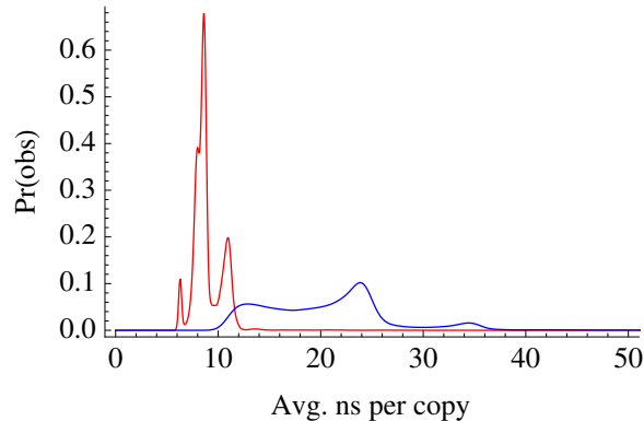
Figure 6.5: Smooth histogram of 10^6 data points each representing timed averages of 500 copy operations, first on the same NUMA node (red line) and then across different NUMA nodes (blue line). The performance of a copy on the same NUMA node seems to be much more consistent.
