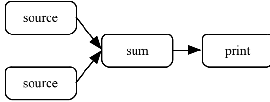
Figure 3.1: Simple streaming application example with four compute kernels of three distinct types. From left to right: the two source kernels each provide a number stream, the “sum” kernel adds pairs of numbers and the last kernel prints the result. Each kernel acts independently, sharing data via communications streams depicted as arrows.
