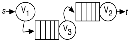
(c) The queueing network G_Q that arises from the topology depicted in Figure 4.2b
