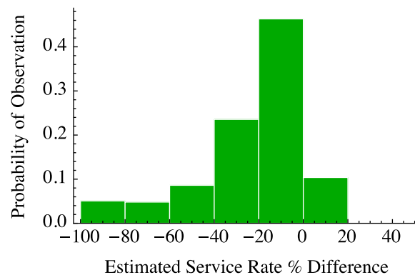
Figure 6.15: Histogram of the probability of estimating the service rate of Kernel B from Figure 6.3. Each execution is a data point, with the percent difference calculated as \left(\frac{\text{observed rate} - \text{set rate}}{\text{set rate}}\right) \times 100 . Not plotted are four outliers to the right of the plotted data which are greater than 1000% difference, which is not unexpected given the probabilistic nature of our heuristic.
